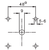
Mounting hole Mounting screw: S3631N M=1,2-1,4 Nm
