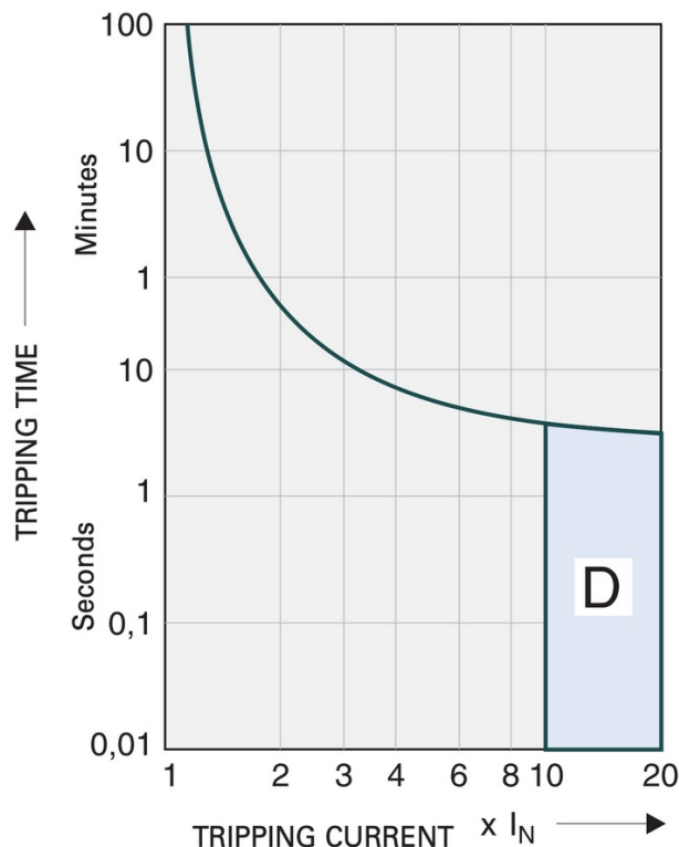
Tripping characteristic D
