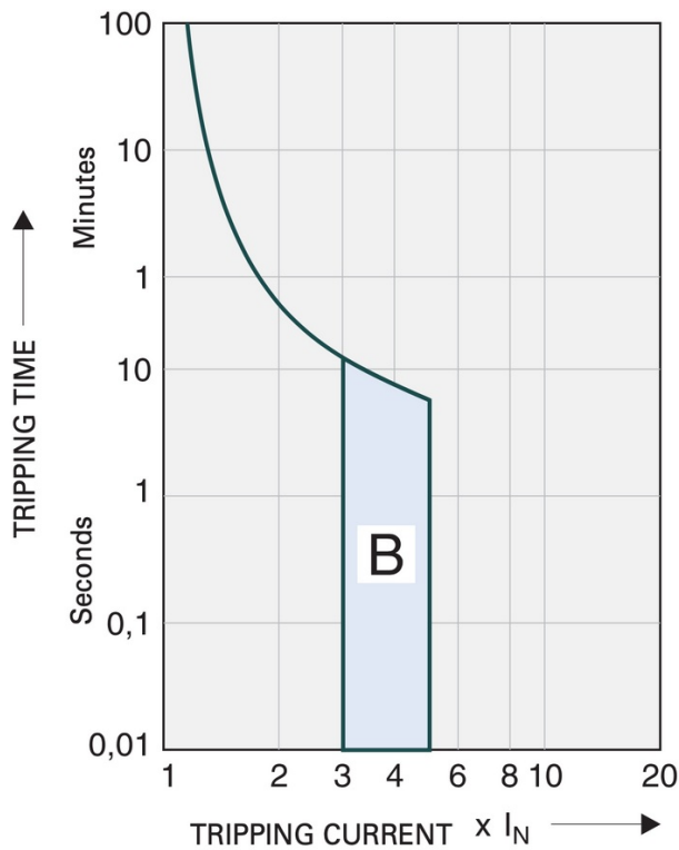
Tripping characteristic B
